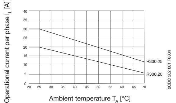
Derating curve
