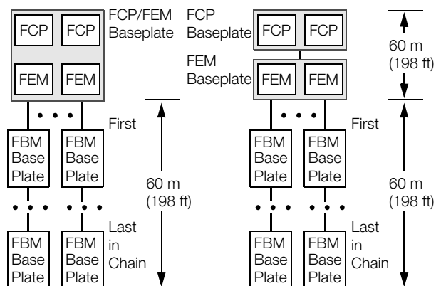
Figure 6. Expanded Fieldbus Cable Length Restrictions
